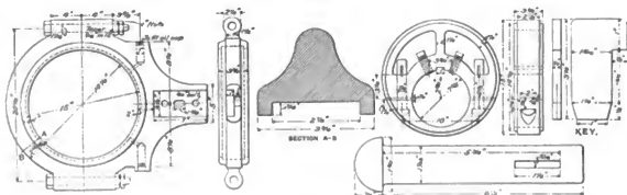
Figs. 1891-1898. Eccentric and Strap for Ten-Wheel (4-6-0) Locomotive. Mexican Centrál.
